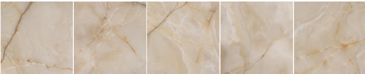
Sovereign Grey
